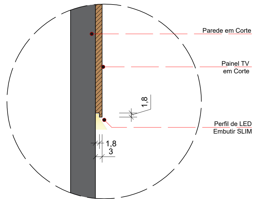
DETALHE 01 - FITA DE LED PAINEL TV
